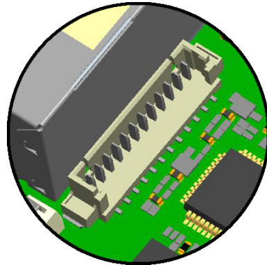
Fig. 27: Molex Audio Connector Detail
