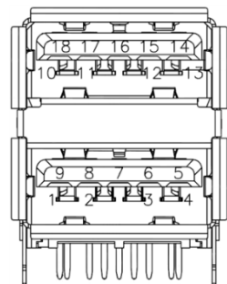
Fig. 18: Dual-USB 3.1 Port Schematic
