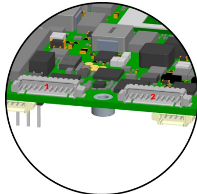
Fig. 51: Molex RS232/485 Connector Detail
