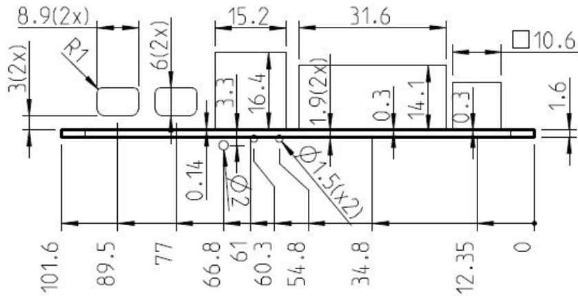
Fig. 5: Recommended cutouts front panel
