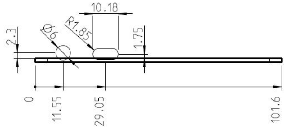
Fig. 7: Recommended cutouts rear panel
