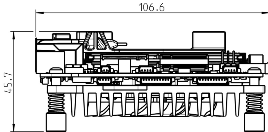
Fig. 13: Dimensions side
