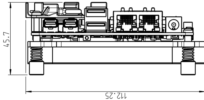
Fig. 12: Dimensions front side
