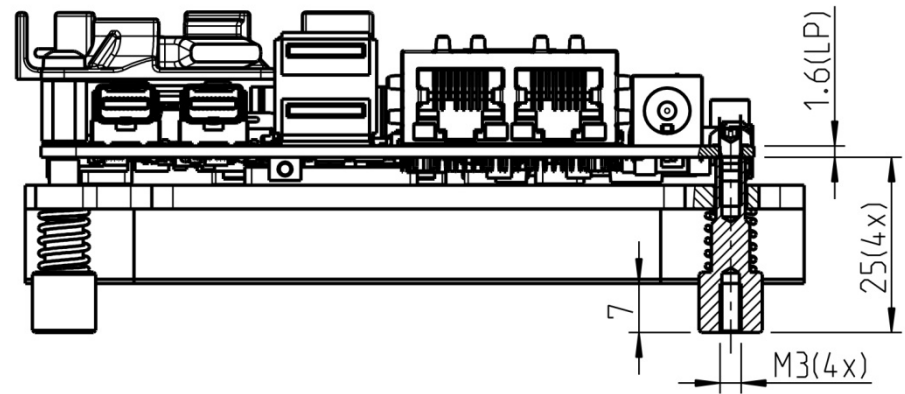
Fig. 14: Dimensions threaded bolts
