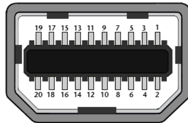
Fig. 16: Mini-DP Connector Schematic
