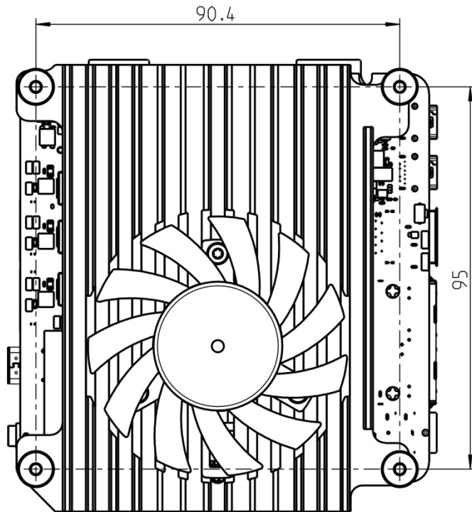
Fig. 10: Dimensions bottom side
