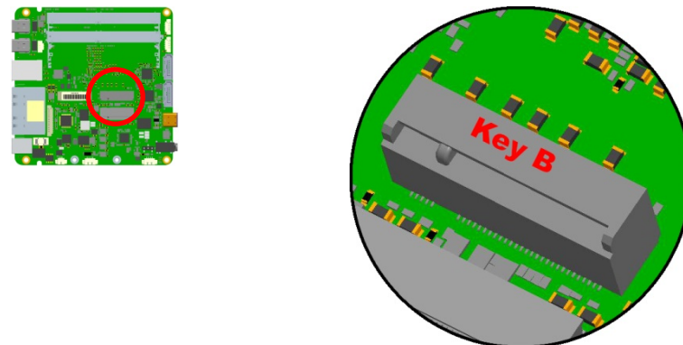
Fig. 31: M.2 Key B Connector Detail
