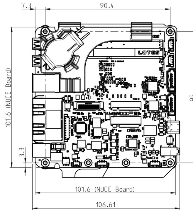
Fig. 11: Dimensions top side
